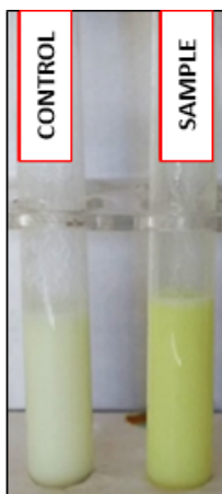
DMAB Test FSSAI (2016)
