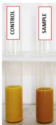
Iodine Test (Milk) Sharma et al. (2012)
