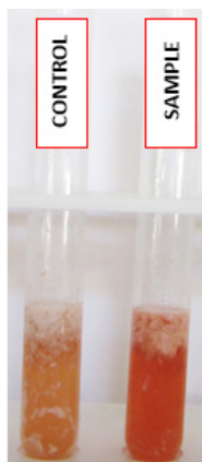
Seliwanoff Test Srivastava (2010)
