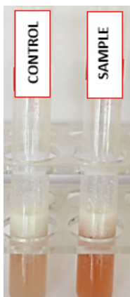
Seliwanoff Test (Milk) Modified- AAU (2018)
