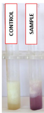
Leach Test (Milk) Modified- AAU (2018)
