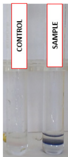
Diphenylamine Test Modified- AAU (2018)
