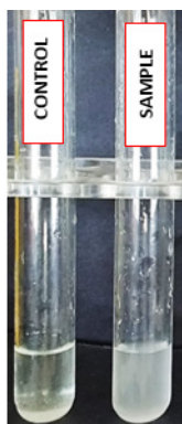
Barium Chloride Test FSSAI (2016)
