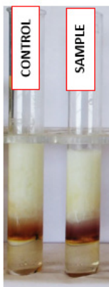
Hehner Test Draaiyer (2009)
