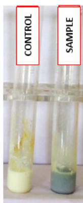
Iodine Test (Milk) Modified- AAU (2018)
