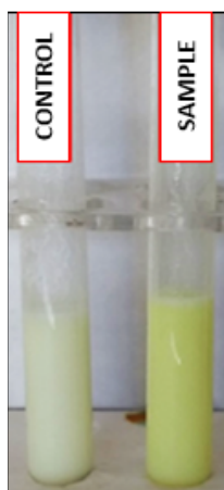
DMAB Test (Milk) Modified- AAU (2018)
