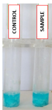
Barfoed Test Barfoed (1873)
