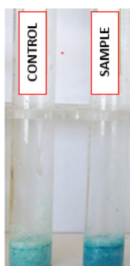
Modified Barfoed Test FSSAI (2016)
