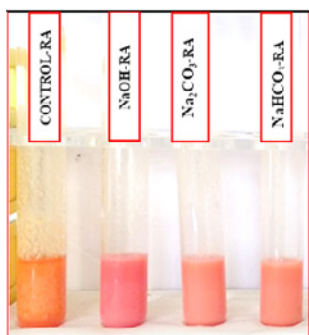
Rosolic acid Test DGHS (2005)
